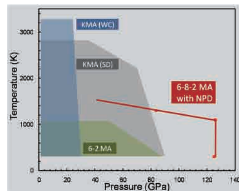
Fig. 1. Pressure-temperature limits in various types of multianvil apparatus. KMA (WC), Conventional Kawai type multianvil apparatus with tungsten carbide anvils (e.g. Irifune et al., 1992); KMA (SD), Kawai type multianvil apparatus with sintered diamond anvil (e.g. Ito, 2007); 6-2 MA, 6-2 type multianvil system (Utsumi and Aoki, 2003); 6-8-2 MA, 6-8-2 type multianvil system (present study).
